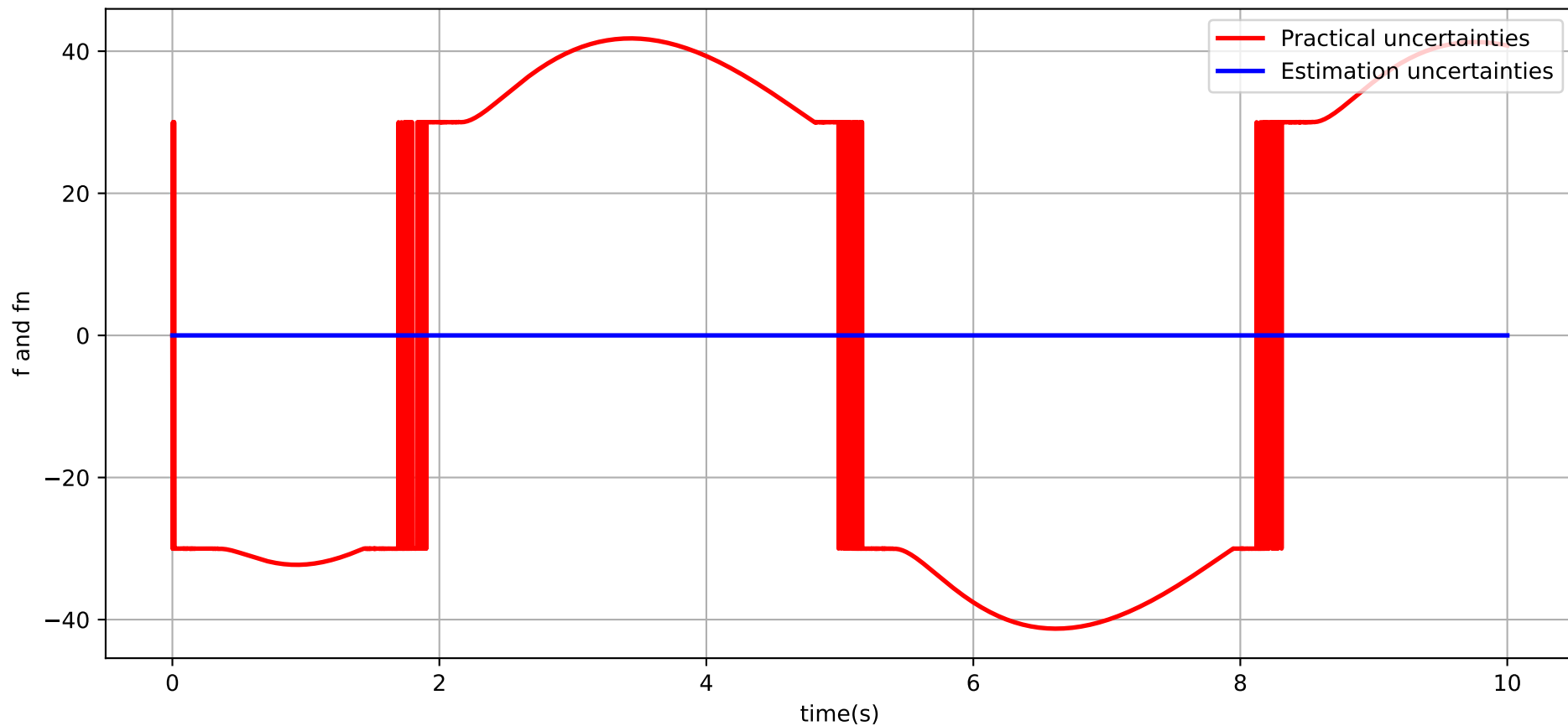
Disturbance Estimation Performance ( S=1 , S1=1 , m=19 )
